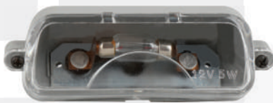
REAR REGISTRATION PLATE LAMP 12V PART NO. SHINX-1309
